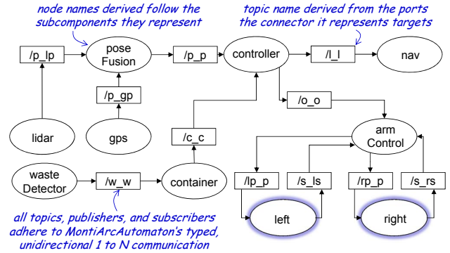
Fig. 3. ROS graph of the cleaning robot architecture depicted in Fig. 3.
