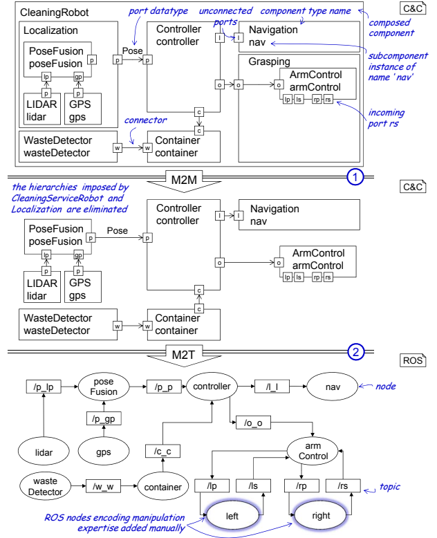
Fig. 2. C&C architecture of a cleaning robot with two arms (top), after applying the M2M transformations for hierarchy elimination (middle), and after applying the M2T transformations producing ROS nodes and topics (bottom).
