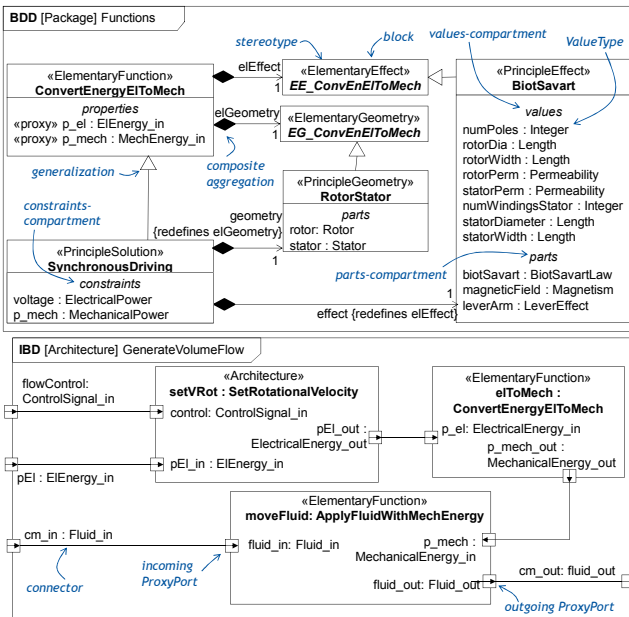
Figure 2: Top: SysML Block Definition Diagram (BDD) of the functional architecture of the running example. Bottom: Internal Block Diagram (IBD) of GenerateVolumeFlow. For details on stereotypes and contents see Sections 4 to 6.
