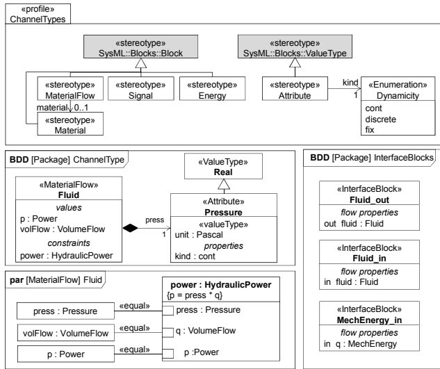
Figure 6: Top: SysML4FMArch’s encoding of the meta-model in Figure 3. Bottom: Examples for channel types modeled in SysML4FMArch.
