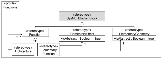
Figure 7: SysML encoding of functions as defined by the meta-model in Figure 4.
